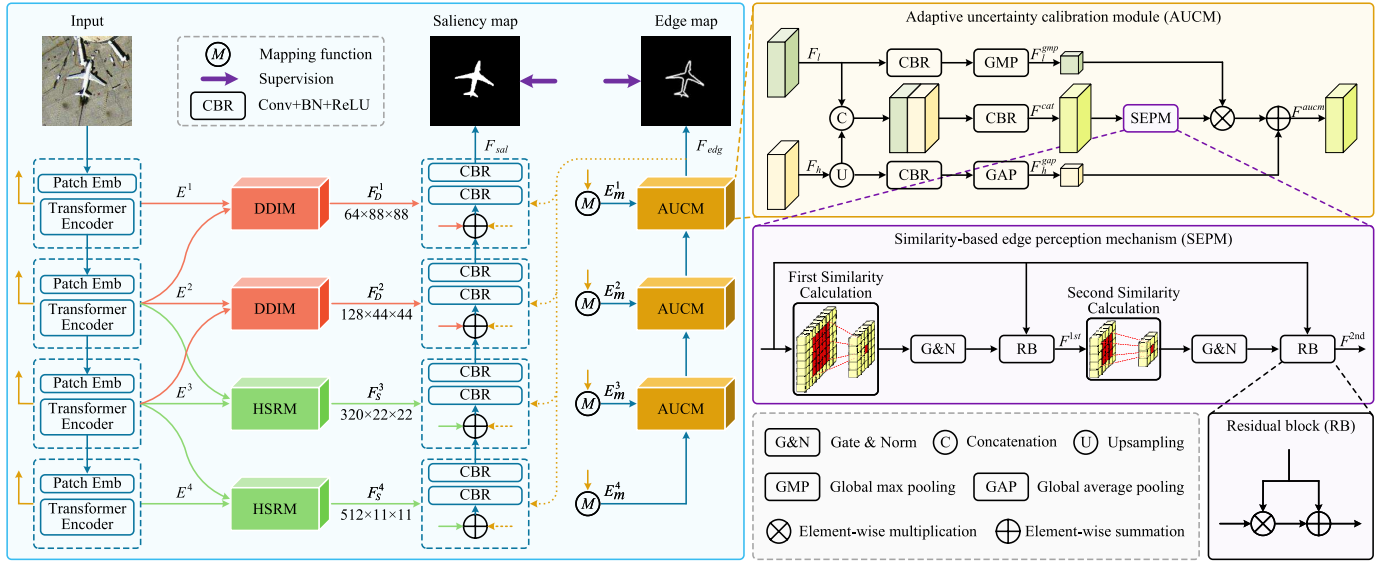
Fig. 2. Architecture of the proposed ERNet. The network mainly consists of saliency prediction branch and edge guidance branch. The former embeds DDIM and HSRM in the skip connections to refine local detail and global semantic, while the latter extracts edge information with pixel similarity and guides saliency prediction branch through the edge decoder composed of cascaded AUCM.
