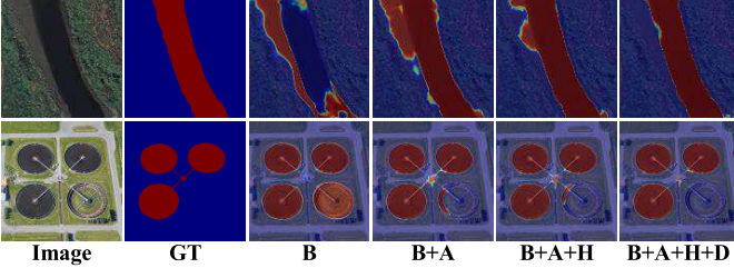
Fig. 8. Visual comparison of different proposed modules in ablation experiments. B, B + A, B + A + H, and B + A + H + D denote baseline, baseline + AUCM, baseline + AUCM + HSRM, and baseline + AUCM + HSRM + DDIM, respectively.
