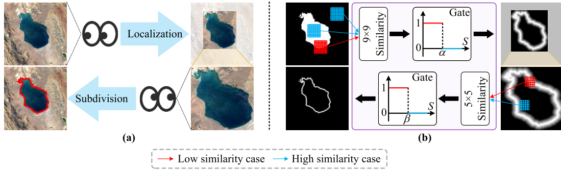
Fig. 1. Main idea of our proposed SEPM. (a) Way humans identify the edge of salient objects. (b) Imitating human behavior through similarity calculation and gating.
