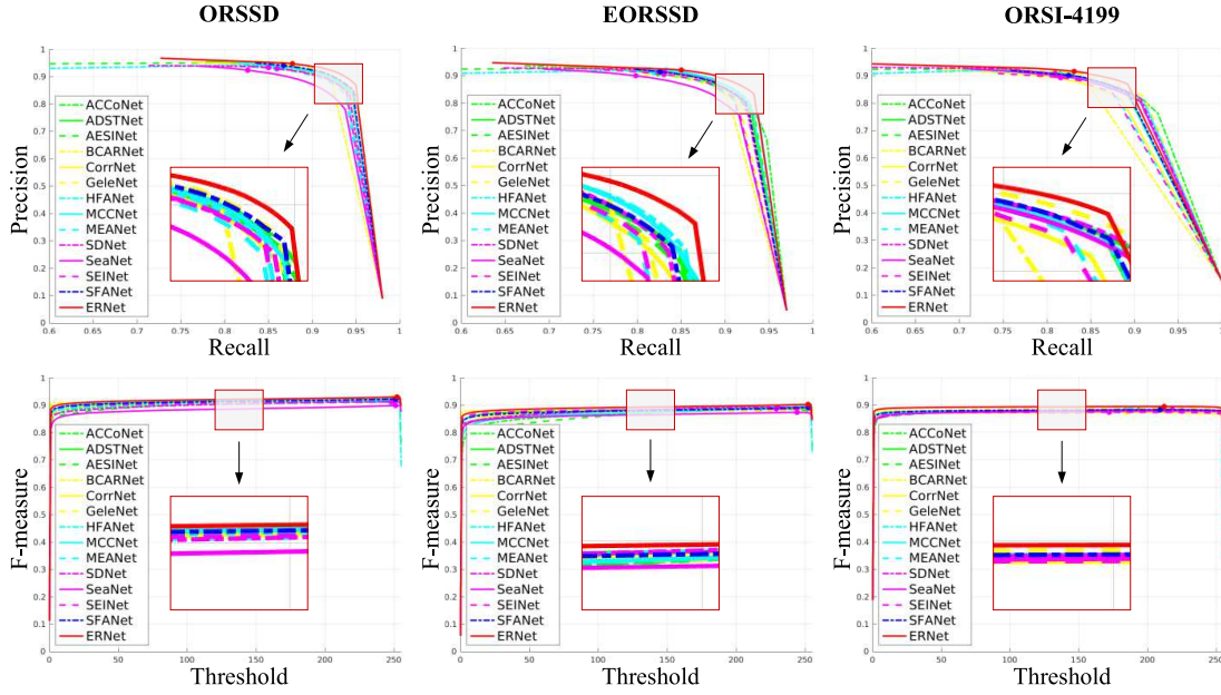
Fig. 6. Comparisons with other methods in terms of PR and F-measure curves on three benchmark datasets.
