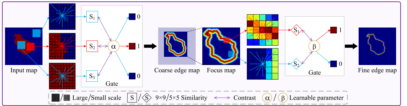
Fig. 3. Illustration of SEPM. In these two stages, this mechanism generates coarse and fine edge maps through similarity calculation from large to small scales and gating mechanisms with learnable thresholds of \alpha and \beta .
