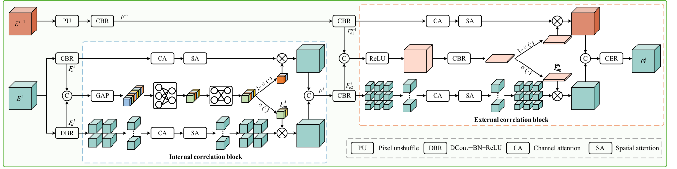
Fig. 4. Illustration of HSRM.
