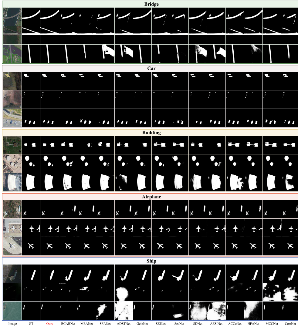
Fig. 7. Qualitative comparisons of our ERNet and other methods.
